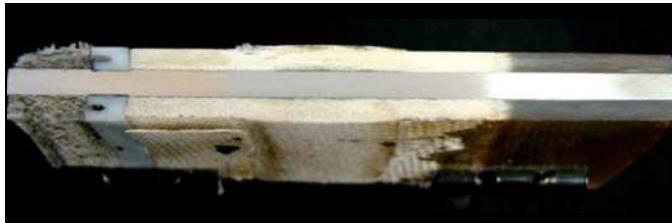
Steam attack on GRE isolation gasket
