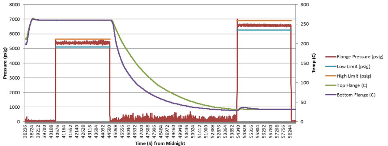
Gasket Sample 5-21-19 - API PR2 Day 1 Test - Test Date: 05-22-2019
