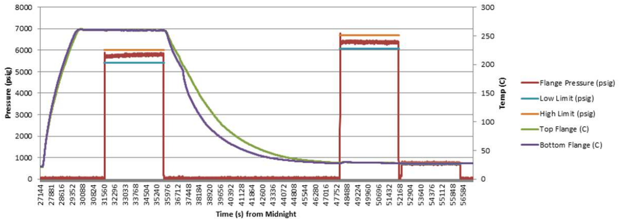
Gasket Sample 5-21-19 - API PR2 Day 3 Test - Test Date: 05-24-2019
