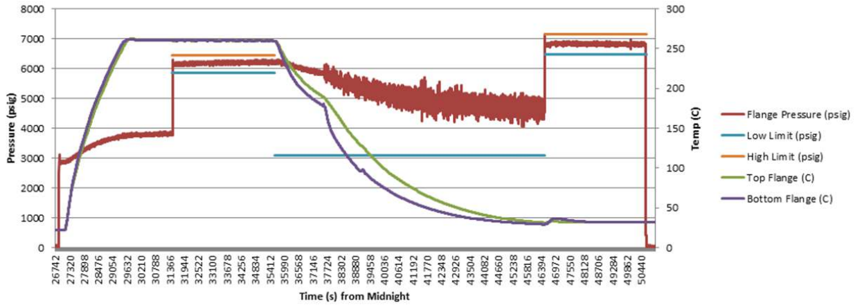
Gasket Sample 5-21-19 - API PR2 Day 2 Test - Test Date: 05-23-2019
